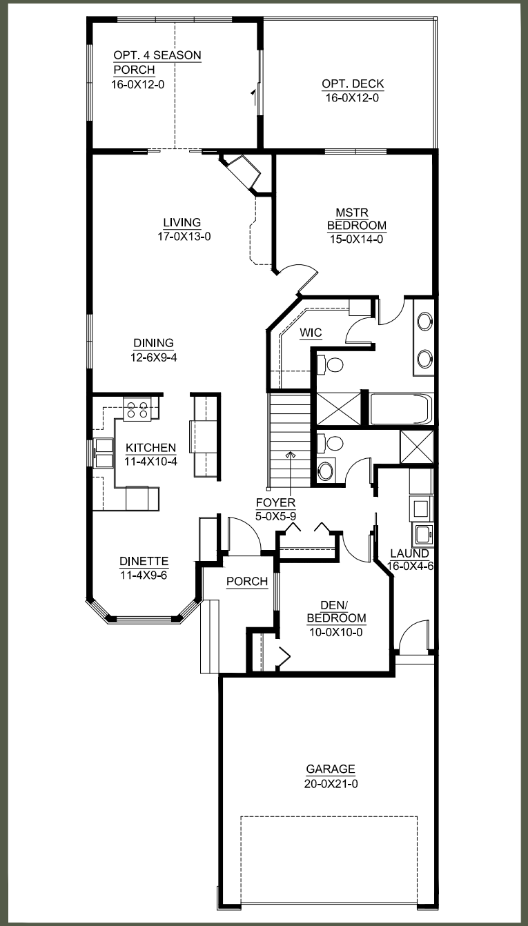
UPPER LEVEL 1,605 finished sq. ft. 2
